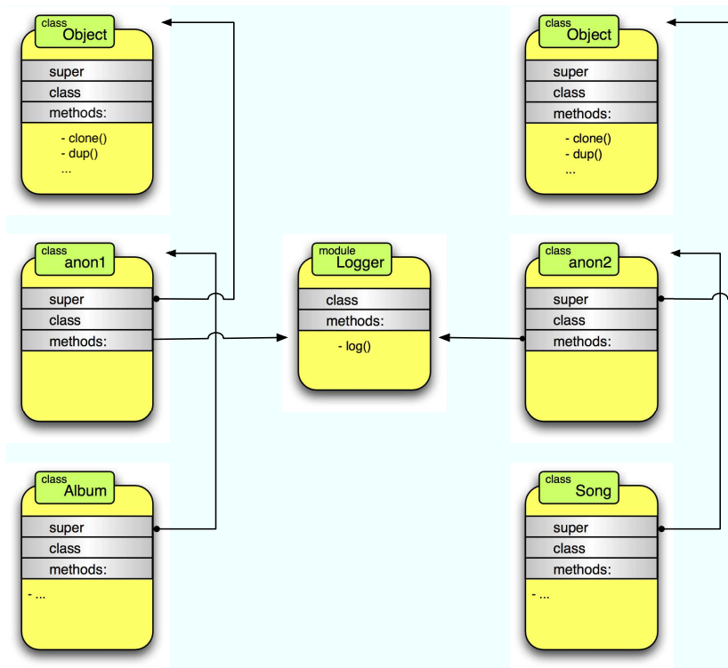
Figure 24.5: How modules are included
