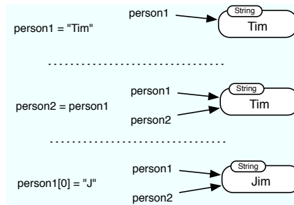
Figure 3.1: Variables hold object references.
