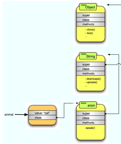
Figure 24.2: Object model for a singleton class
