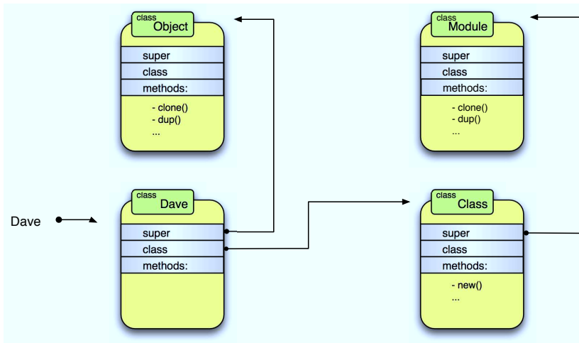
Figure 24.3: Basic class definition
