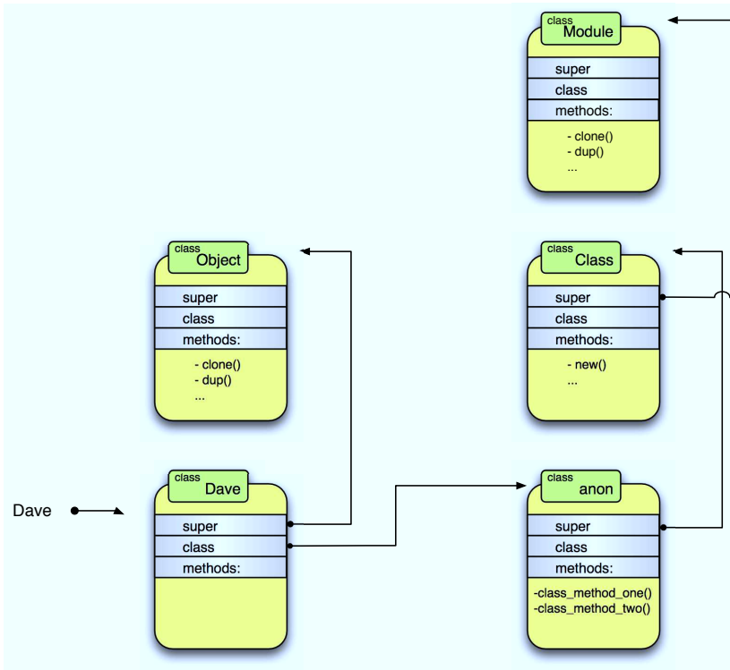
Figure 24.4: Class with so-called class methods
