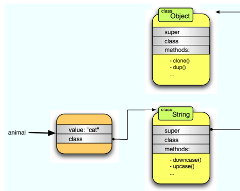
Figure 24.1: Object model for a basic class
