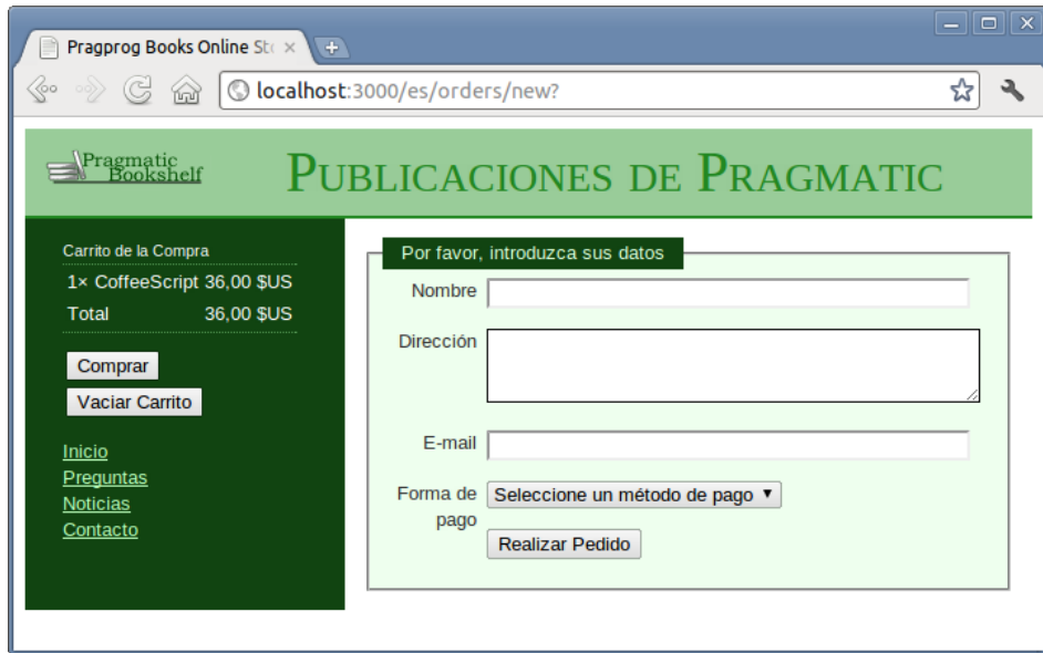
Figure 35—Ready to take your money—in Spanish
