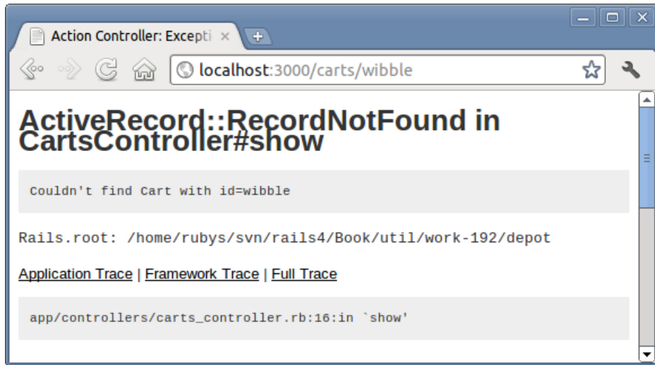
Figure 16—Our application spills its guts.
