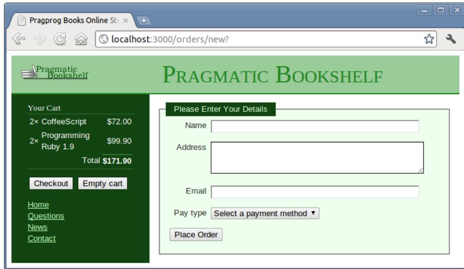
Figure 23—Our checkout screen
