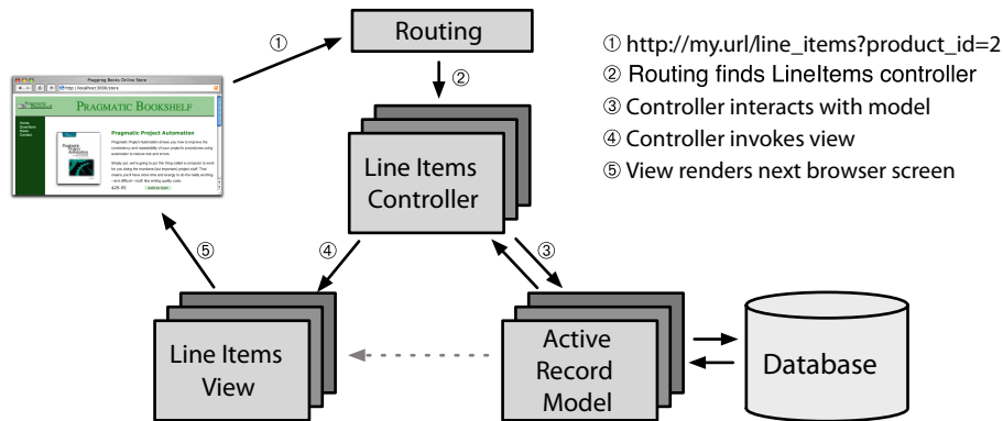
Figure 5—Rails and MVC
