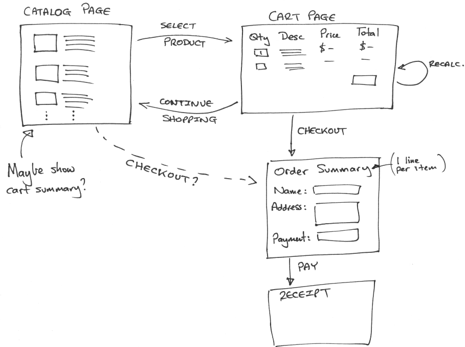
Figure 6—Flow of buyer pages
