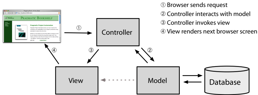
Figure 4—The Model-View-Controller architecture
