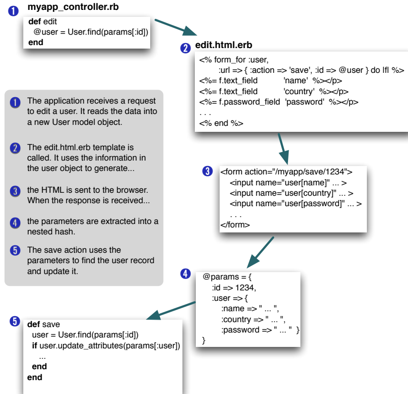
Figure 49—Models, controllers, and views work together.
