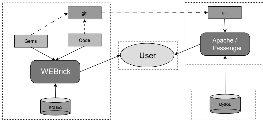
Figure 41—Application deployment road map
