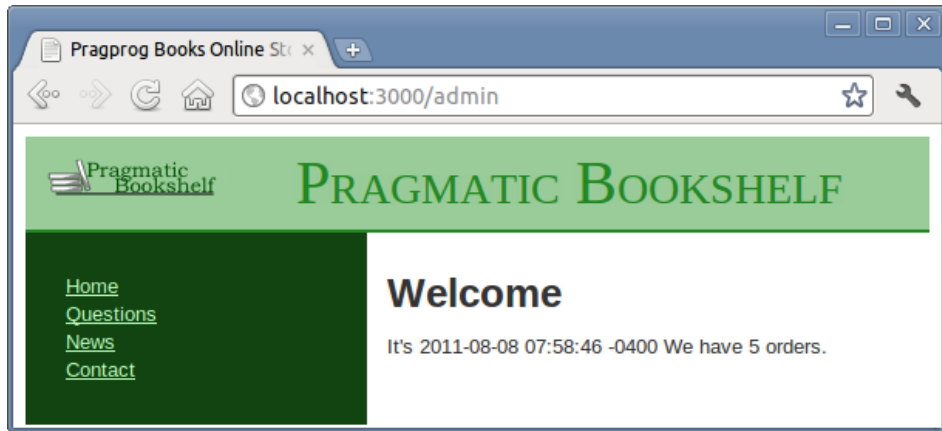
Figure 29—Administrative interface
