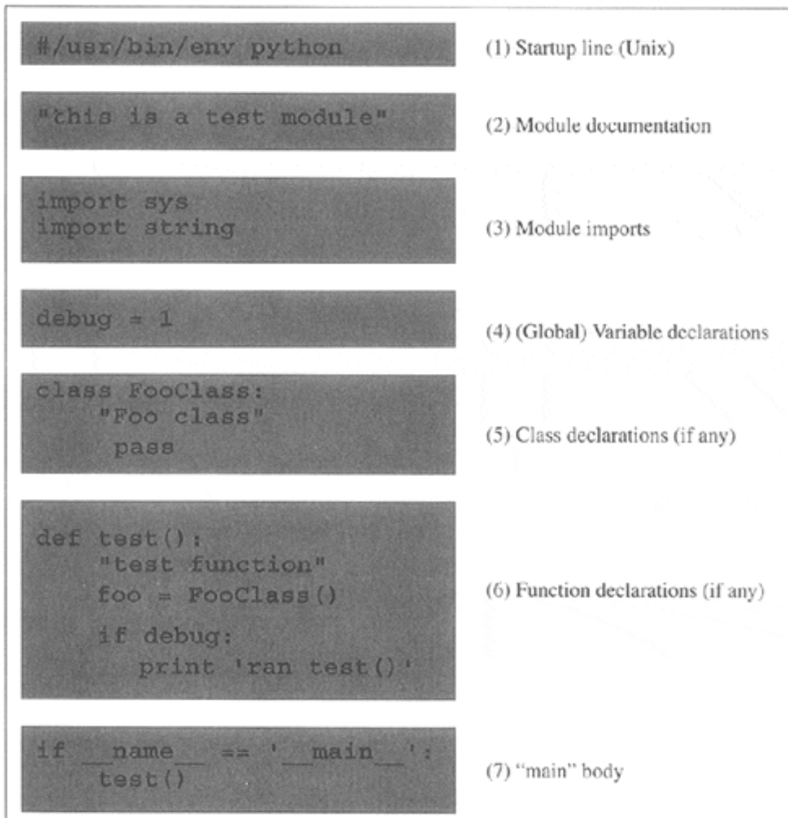
Figure 3-1. Typical Python File Structure
