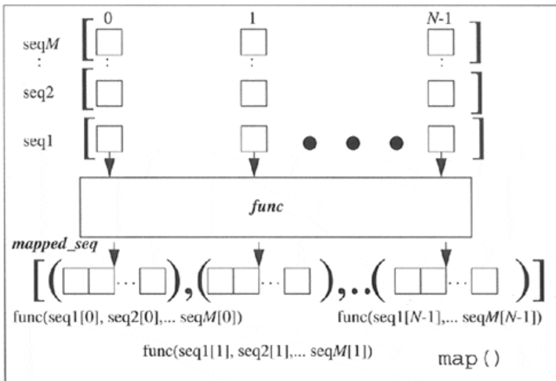
Figure 11-3. How the map() Built-in Function Works with > 1 Sequence
