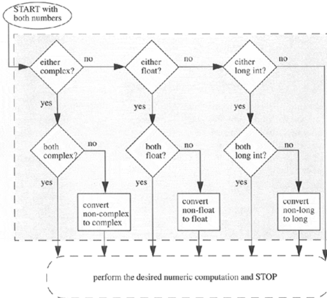
Figure 5.1. Numeric coercion.
