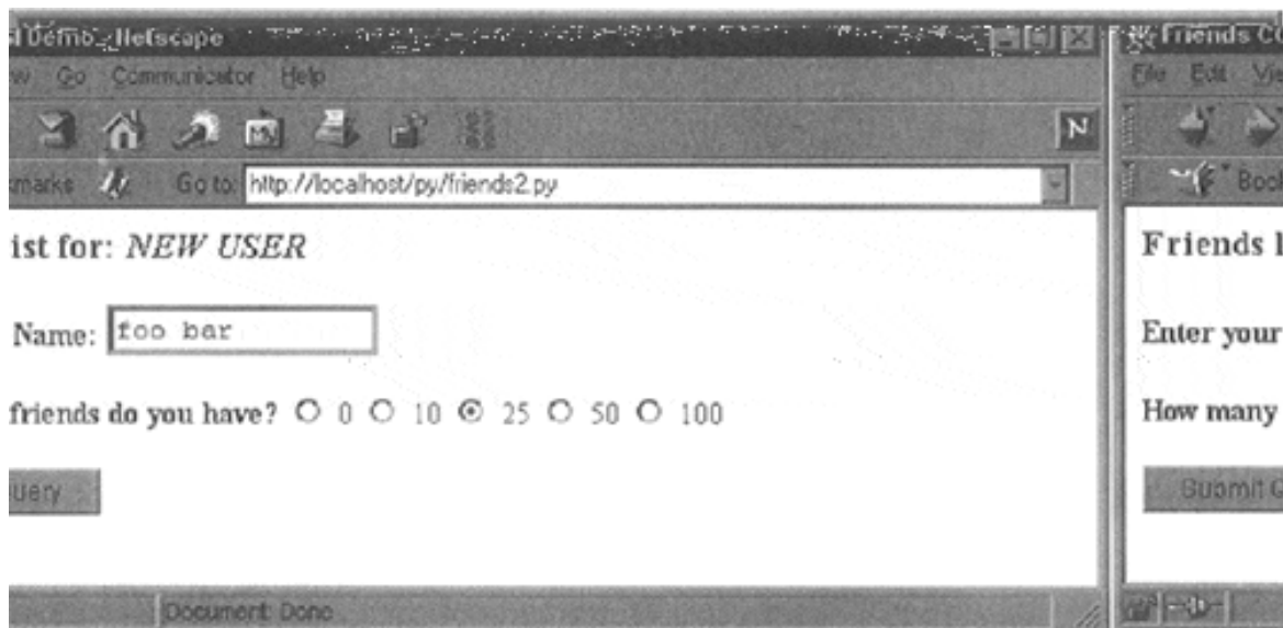
Figure 19-7. Friends Results Page in Netscape4 on Windows
