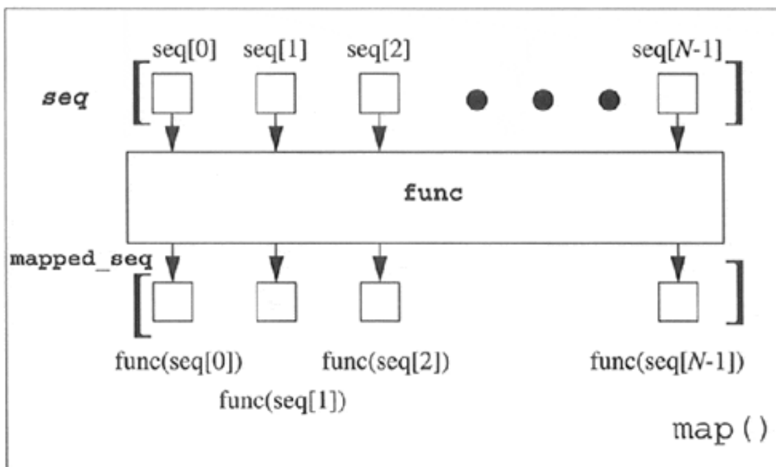
Figure 11-2. How the map( ) Built-in Function Works
