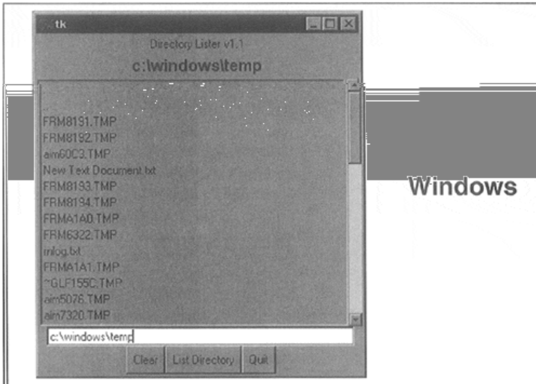
Figure 18-5. List Directory GUI Application in Windows (listdir.py)
