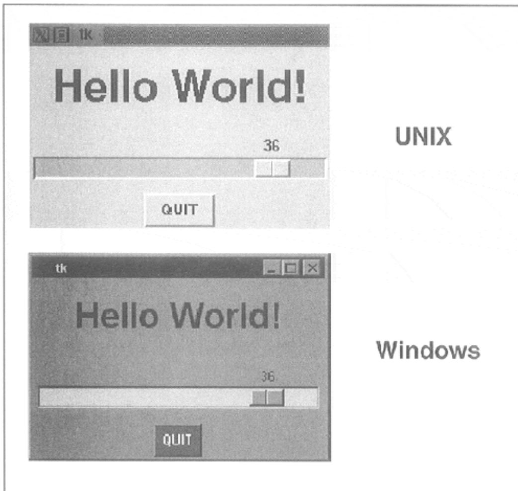
Figure 18-4. Tkinter Label, Button, and Scale Widgets (tkhello4.py)
