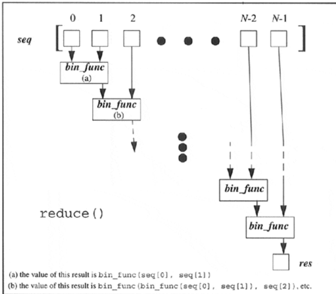
Figure 11-4. How the reduce() Built-in Function Works
