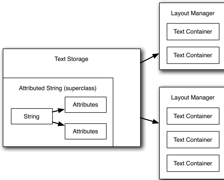
Figure 8.2: The relationship between text storage and layout managers.
