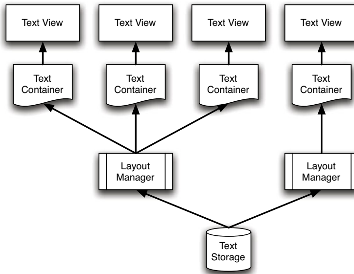
Figure 8.10: The text system arrangement.
