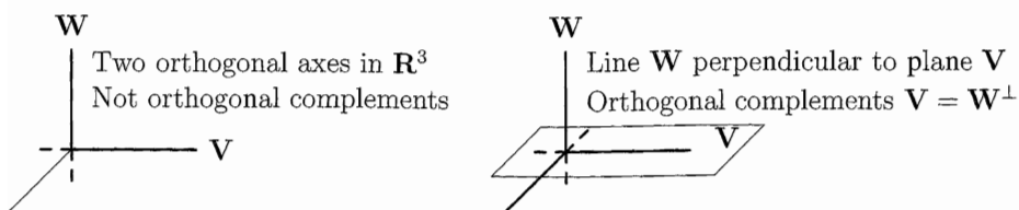
Figure 3.3 Orthogonal complements in \mathbf{R}^3 : a plane and a line (not two lines).
