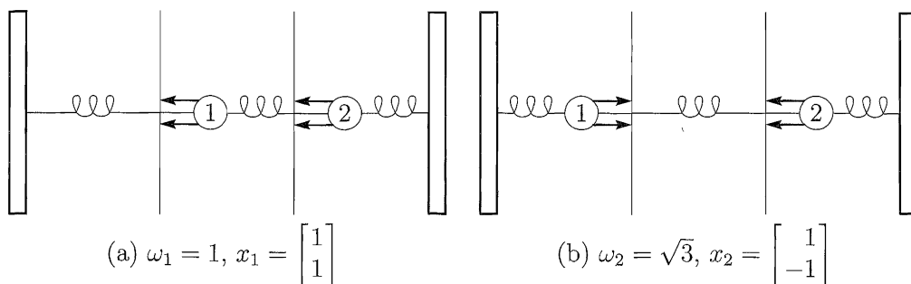
Figure 5.3 The slow and fast modes of oscillation.
