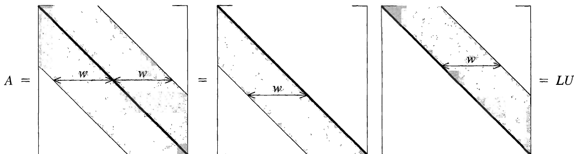
Figure 1.8 A band matrix A and its factors L and U .
