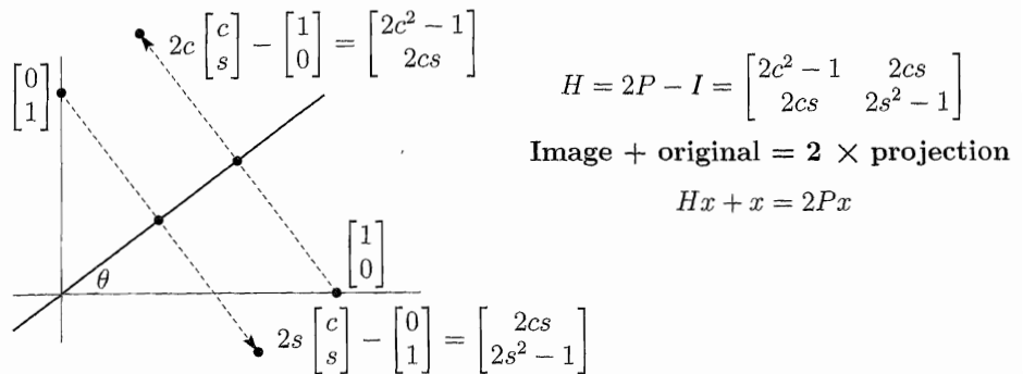
Figure 2.11 Reflection through the \theta -line: the geometry and the matrix.
