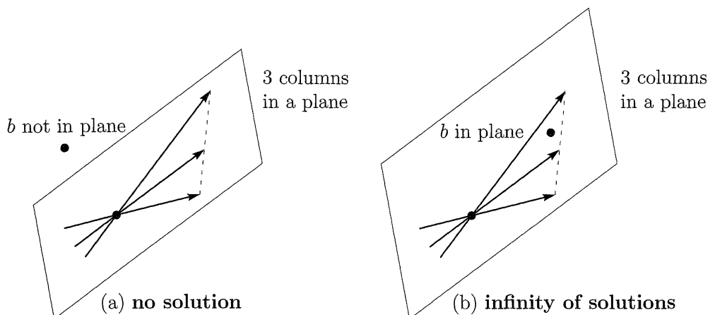
Figure 1.6 Singular cases: b outside or inside the plane with all three columns.
