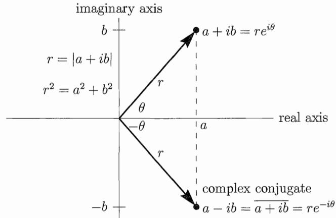
Figure 5.4 The complex plane, with a + ib = re^{i\theta} and its conjugate a - ib = re^{-i\theta} .
