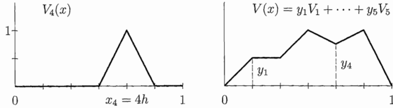
Figure 6.7 Hat functions and their linear combinations.
