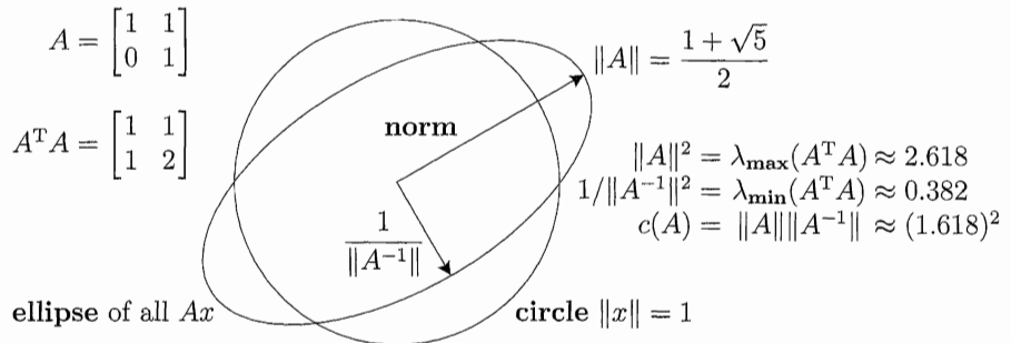
Figure 7.1 The norms of A and A^{-1} come from the longest and shortest Ax .
