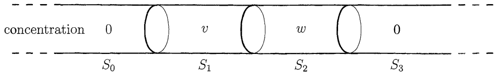
Figure 5.1 A model of diffusion between four segments.
