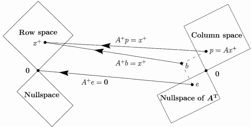
Figure 6.3 The pseudoinverse A^+ inverts A where it can on the column space.
