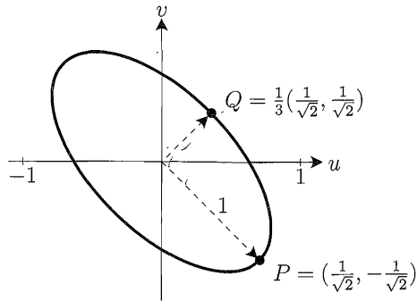
Figure 6.2 The ellipse x^T A x = 5u^2 + 8uv + 5v^2 = 1 and its principal axes.
