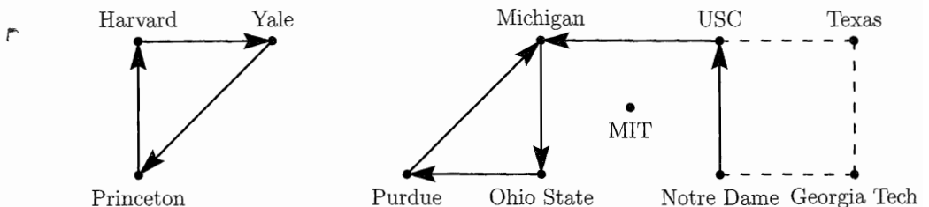
Figure 2.7 Part of the graph for college football.
