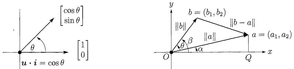
Figure 3.6 The cosine of the angle \theta = \beta - \alpha using inner products.
