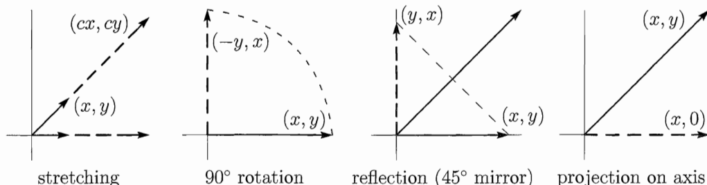
Figure 2.9 Transformations of the plane by four matrices.
