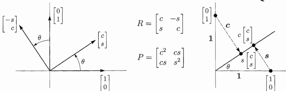
Figure 2.10 Rotation through \theta (left). Projection onto the \theta -line (right).
