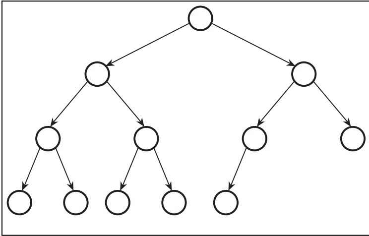
Here is a dense binary tree. Every level is full, except the last level, where the nodes are all packed to the left of the tree.
