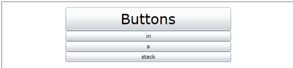
Figure 20-3. Vertical StackPanel
